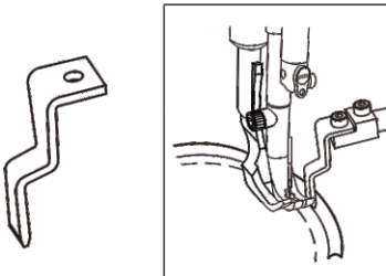
Guiding knife for curve stitch 曲線縫傍刀
