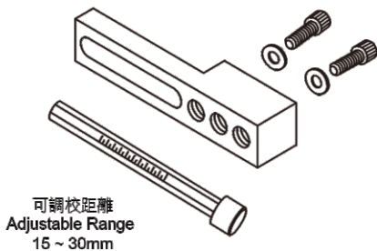
15 - 30mm stitches distance adjustment kit for KG867P KG867P 15 - 30mm 縫線間距調節配件
