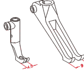
Narrow standard feet 窄身標準壓腳
