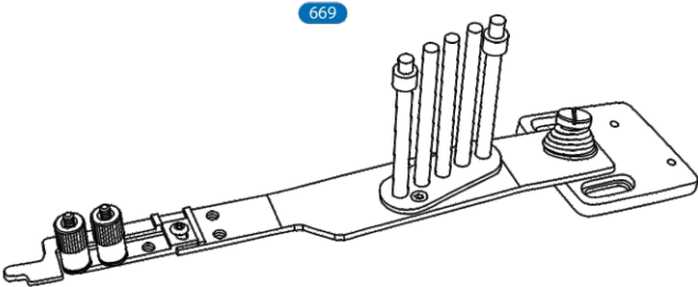
Moving arm for binding 包邊筒擺架
