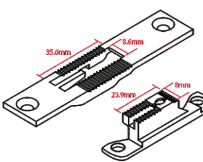
Needle plate & feed dog for thin material 薄料用針板及送布牙
