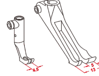
Narrow standard feet with wider right toe 右趾較寬窄身標準壓腳
