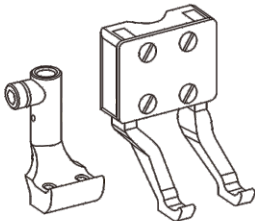
Double needle compensating feet set 雙針高低壓腳組
