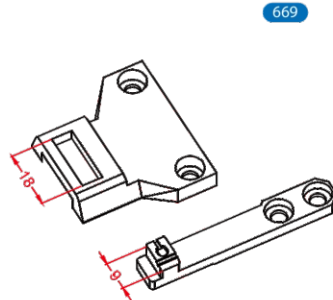
Raised needle plate & feed dog 升高針板及送布牙
