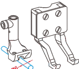
Double needle compensating feet for piping 雙針高低繩管壓腳組
