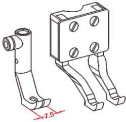
Single needle compensating feet set 單針高低壓腳組
