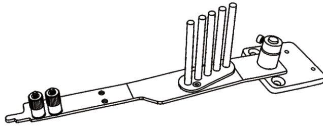
Moving arm for binding on 669 machine (Rocking with feed dog) Use together with KHF2, KHF3 or KHF4 binder 669包邊用送料擺架(跟送布牙擺動)，可配搭KHF2, KHF3或KHF4使用
