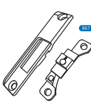
Needle plate & feed dog for binding 包邊用針板及送布牙
