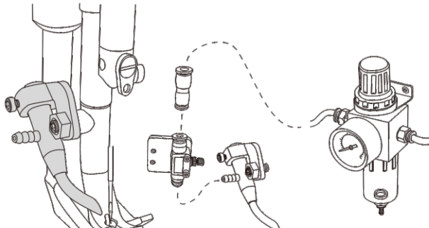
Needle cooler for single needle machine 單針機用車針冷卻裝置
