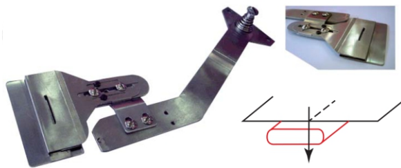
N516-V91174 Tape guide, it is adjustable between 1.5cm & 4cm N516-V91174 導帶器，可調教寬度: 1.5cm - 4cm
