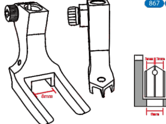
Presser feet for invisible zipper 隱形拉鍊壓腳
