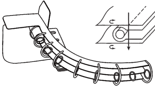
KHF767WL finishes functions of KHF767P1 & KHF767P2 simultaneously KHF767WL能同一時間做到KHF767P1及KHF767P2的效果
