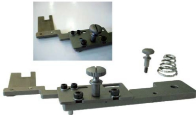
Partition attachment separates the upper and lower layers, to set the upper feeding and lower feeding different from each other 將上下層物料分開，達致不同步推送
