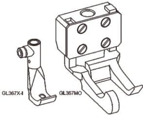
Compensating left guide feet (for extreme heavy) 左傍高低壓腳 (極厚物用)
