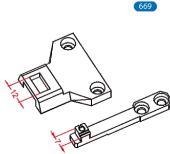
Raised, small needle plate & feed dog 升高短針板及送布牙
