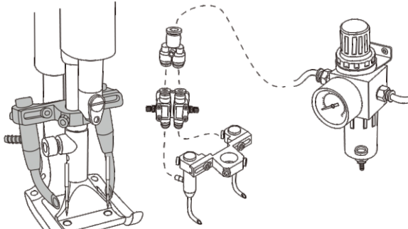
Needle cooler for double needle machine 雙針機用車針冷卻裝置
