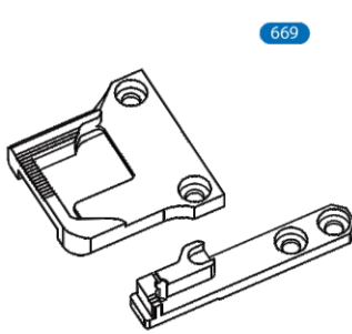
Needle plate & feed dog for binding 包邊用針板及送布牙
