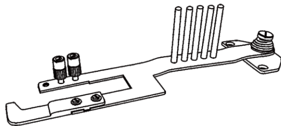
Moving arm for 767 & 867, used together with KHF2, KHF3 or KHF4 binder 767及867包邊筒擺架，配搭KHF2, KHF3或KHF4 使用
